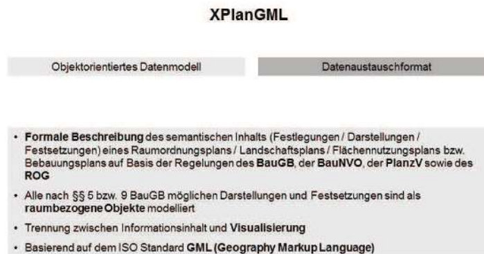
Abb. 2: Standard XPlanGML
